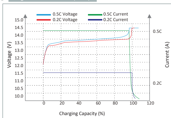
● Charge characteristics (25°C)
