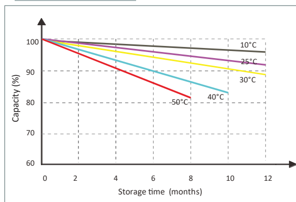
● Self-Discharging Curve
