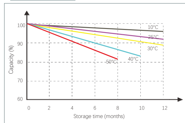
● Self-Discharging Curve
