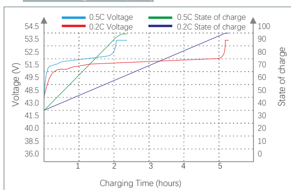
● State of Charge Curve (25°C)
